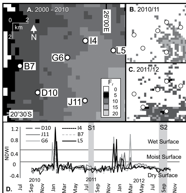
Figure 1. Surface moisture trends (flood frequency, F_f ) assessed by the Moderate Resolution Imaging Spectroradiometer. A: 10 yr of data between 2000 and 2010 (scale is fraction of time between 0% and 20% of time that the playa was inundated). B: Data for year prior to ground measurements (2010–2011). C: Data for year between ground measurements (2011–2012) using the same scale. D: Temporal sequence of surface moisture within 0.25 km 2 area surrounding each site. S1 and S2 indicate study periods; L5, J11, D10, G6, I4, and B7 indicate study sites. NDWI—normalized difference water index.
